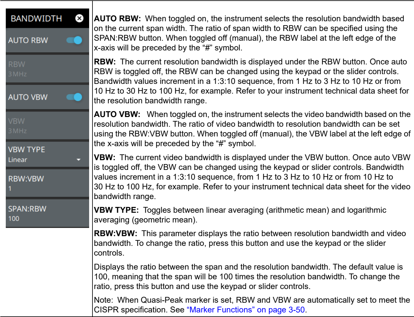
Figure 3-11. BANDWIDTH Menu
