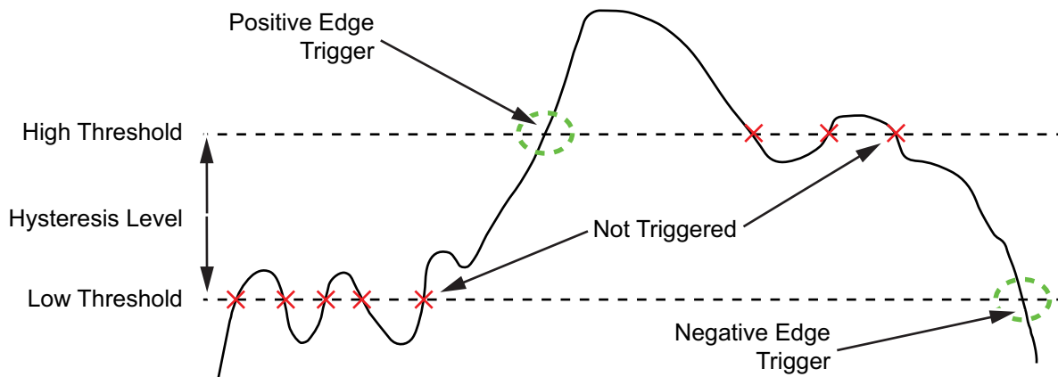
Figure 3-54. Trigger Levels and Hysteresis
