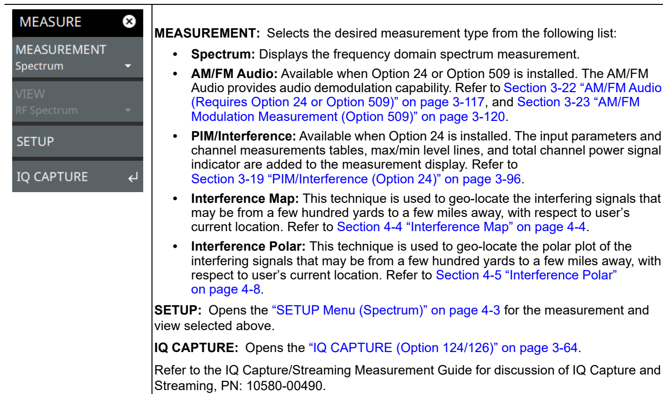
Figure 4-2. MEASURE Menu
