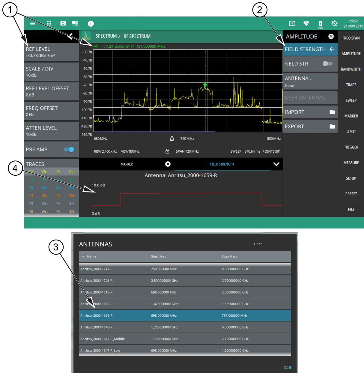
Figure 3-9. Field Strength Measurement (1 of 2)
