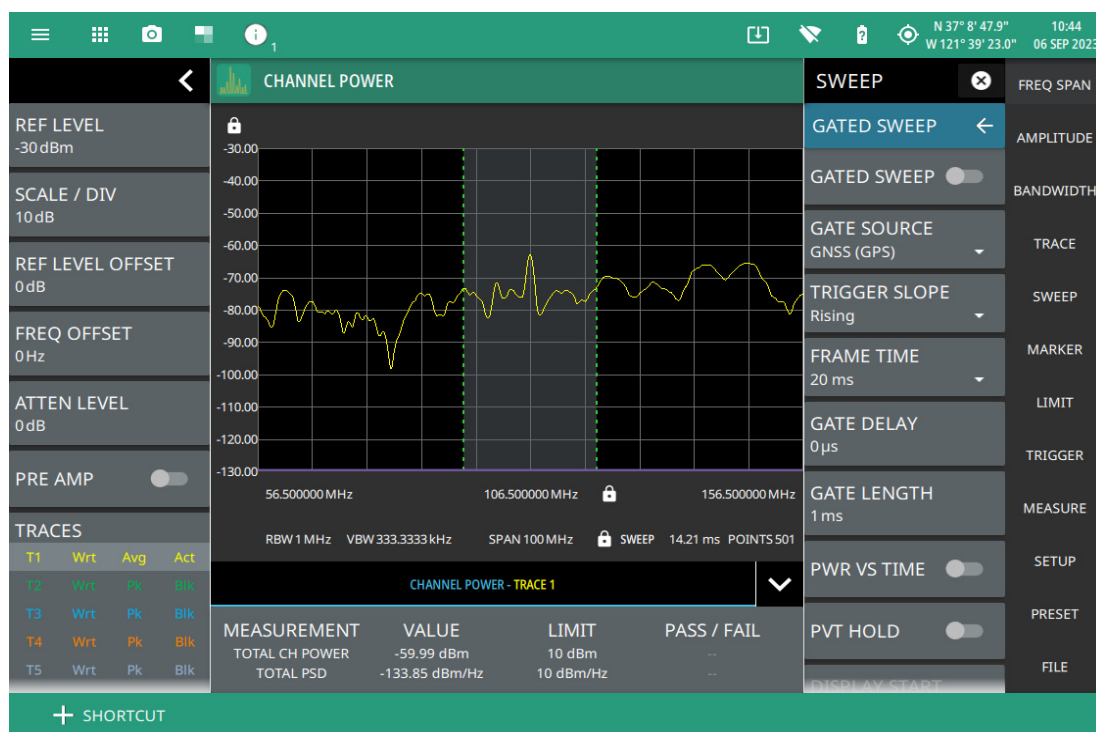
Figure 3-29. Gated Sweep Measurement
