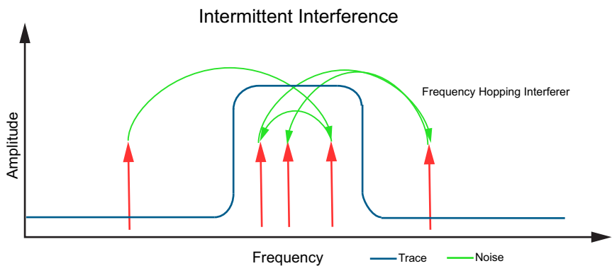
Figure 3-105. Intermittent Interference
