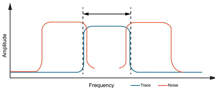
Figure 3-103. Adjacent Interference
