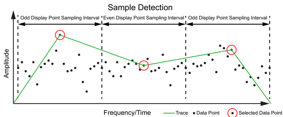
Figure 3-19. Sample Detector Type
