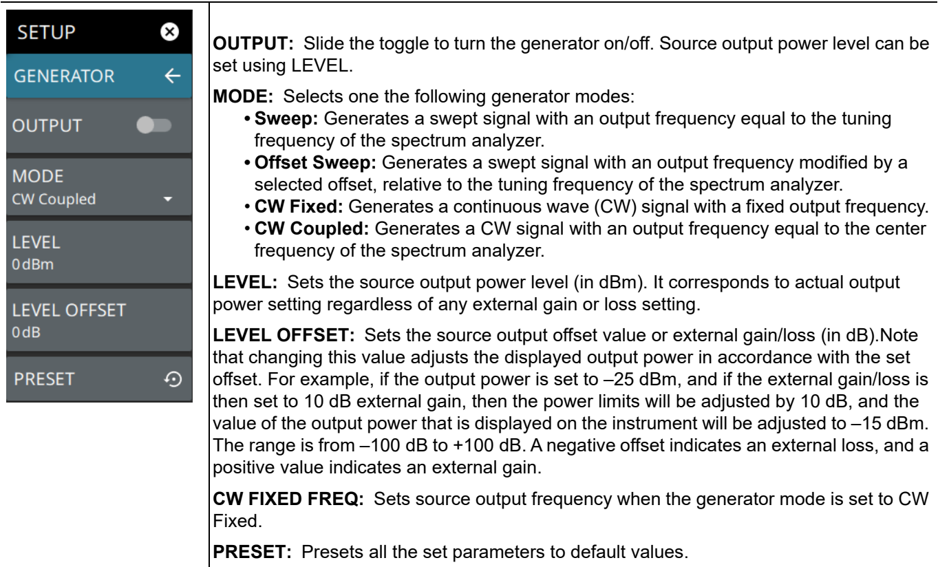
Figure 3-59. GENERATOR Submenu
