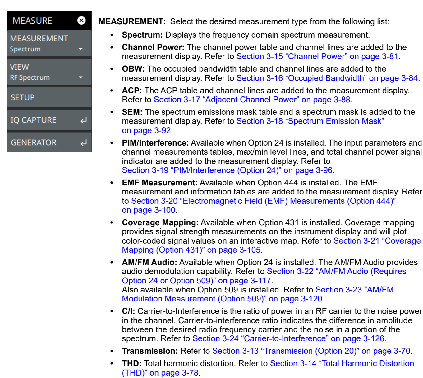
Figure 3-46. MEASURE Menu
