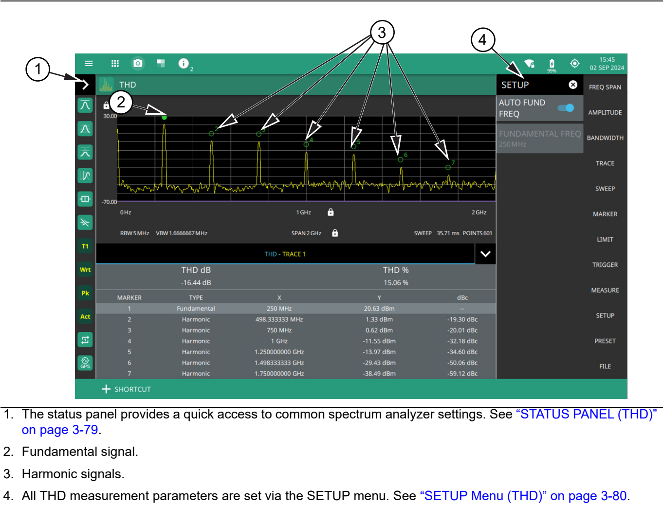
Figure 3-64. THD Measurement
