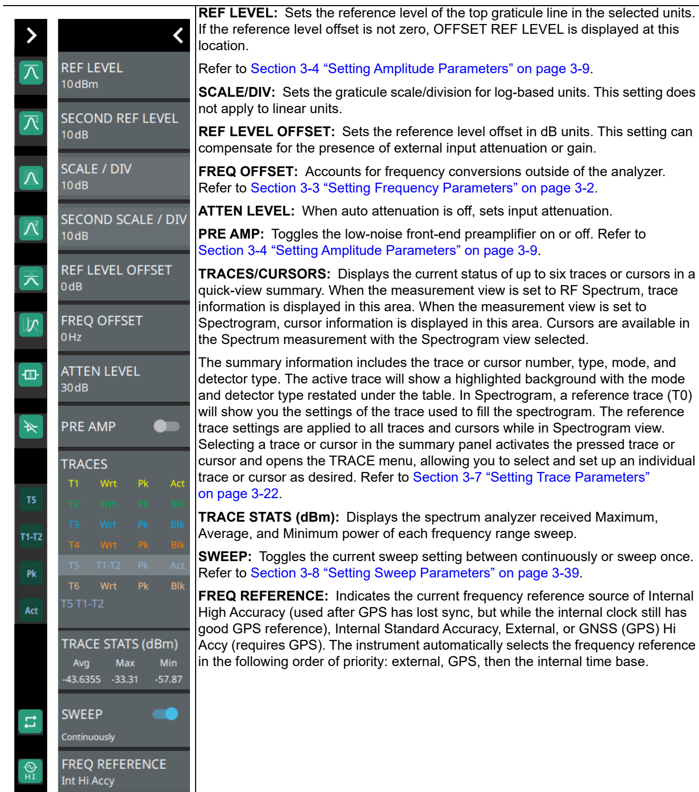
Figure 3-74. Status Panel with Minimized Status Panel Icons (Adjacent Channel Power)
