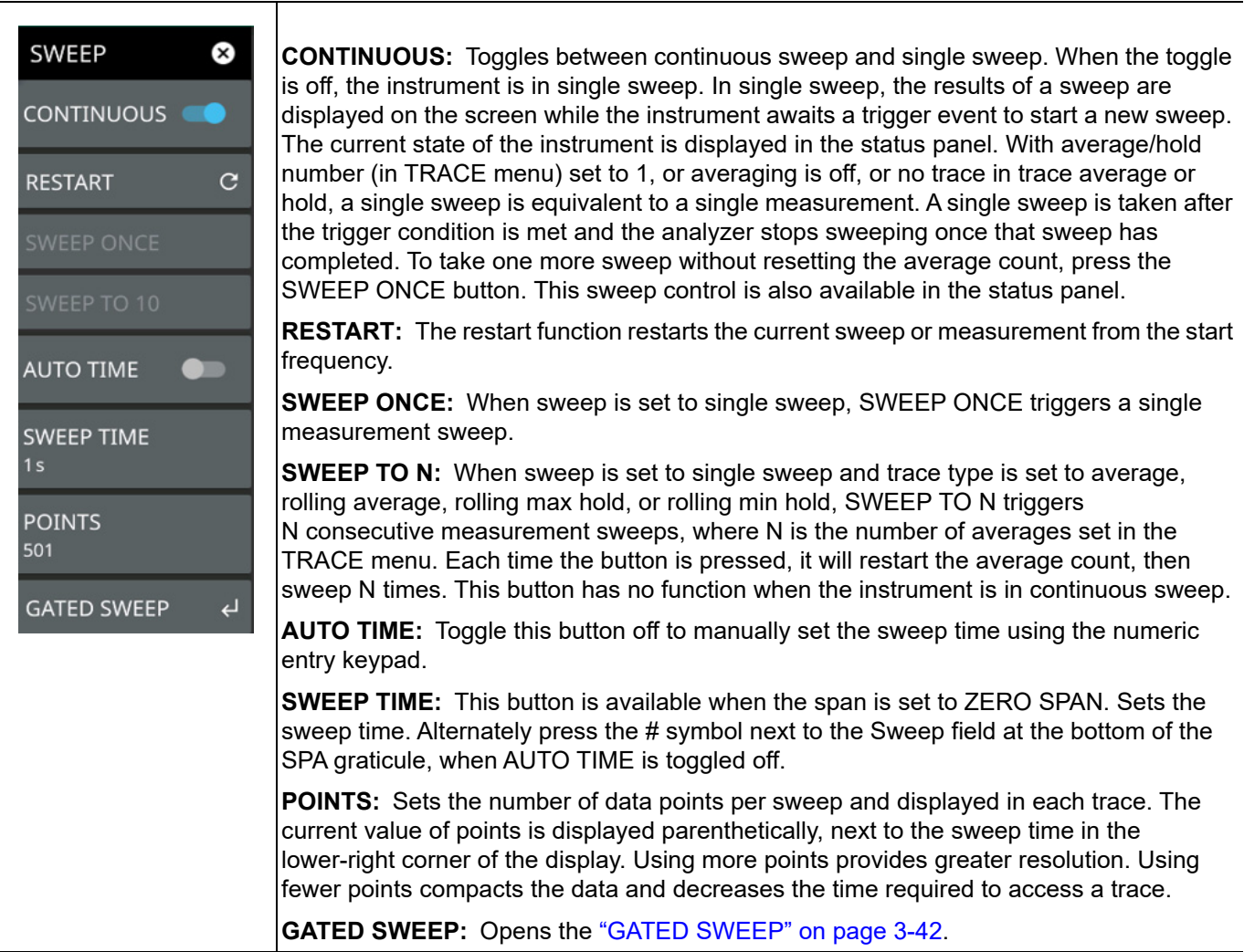
Figure 3-28. SWEEP Menu
