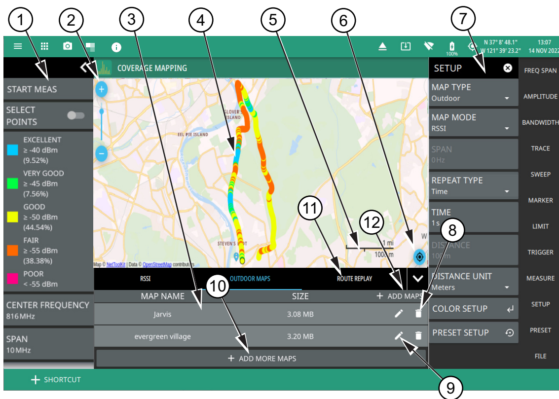
Figure 3-86. Coverage Mapping (Outdoor) (1 of 2)
