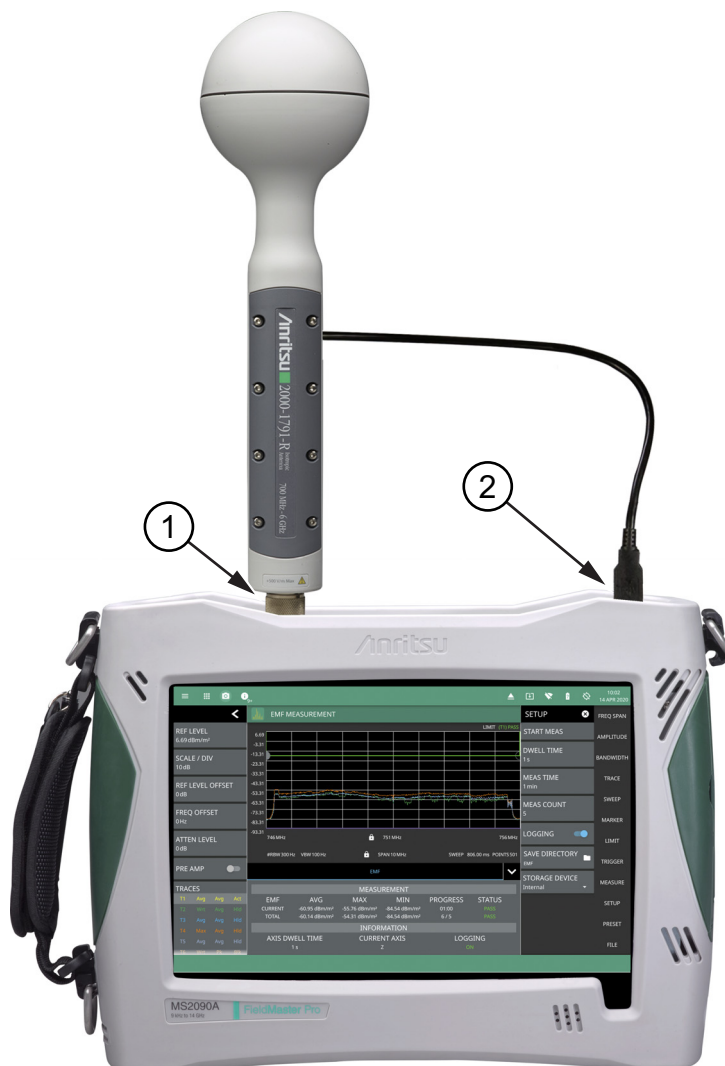
Figure 3-82. Isotropic Antenna Connection
