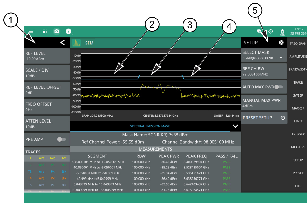
Figure 3-76. SEM Measurement
