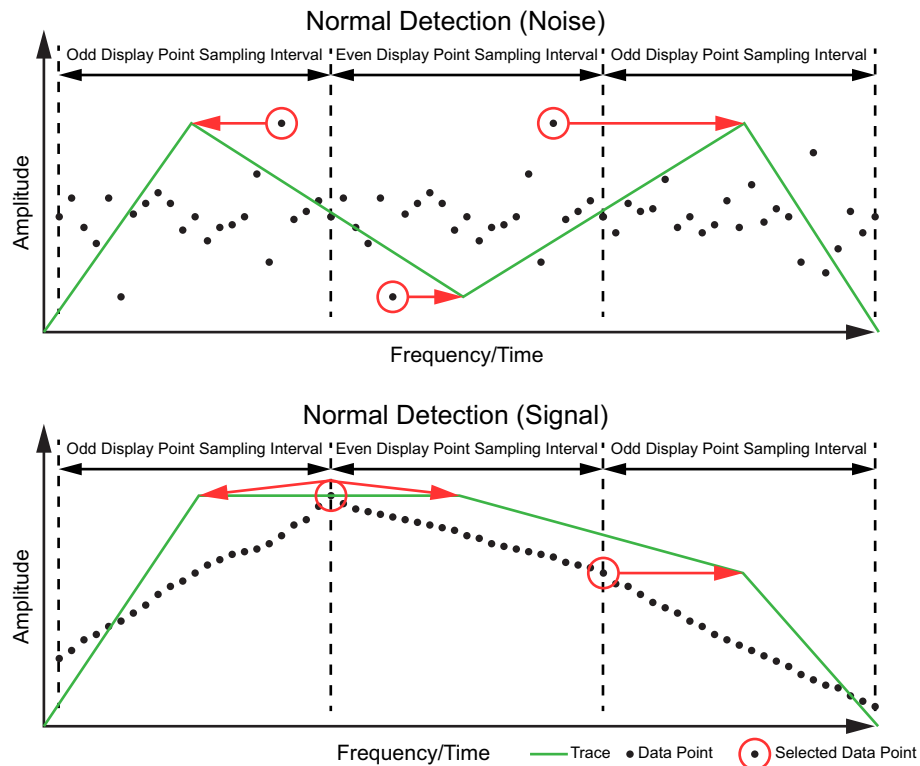
Figure 3-20. Normal Detector Type
