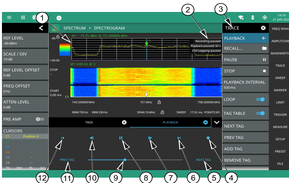
Figure 3-23. Trace Record and Playback (1 of 2)
