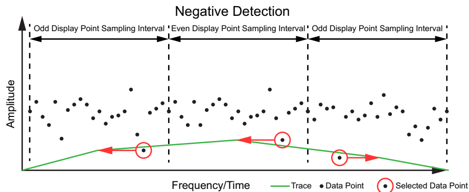
Figure 3-18. Negative Detector Type
