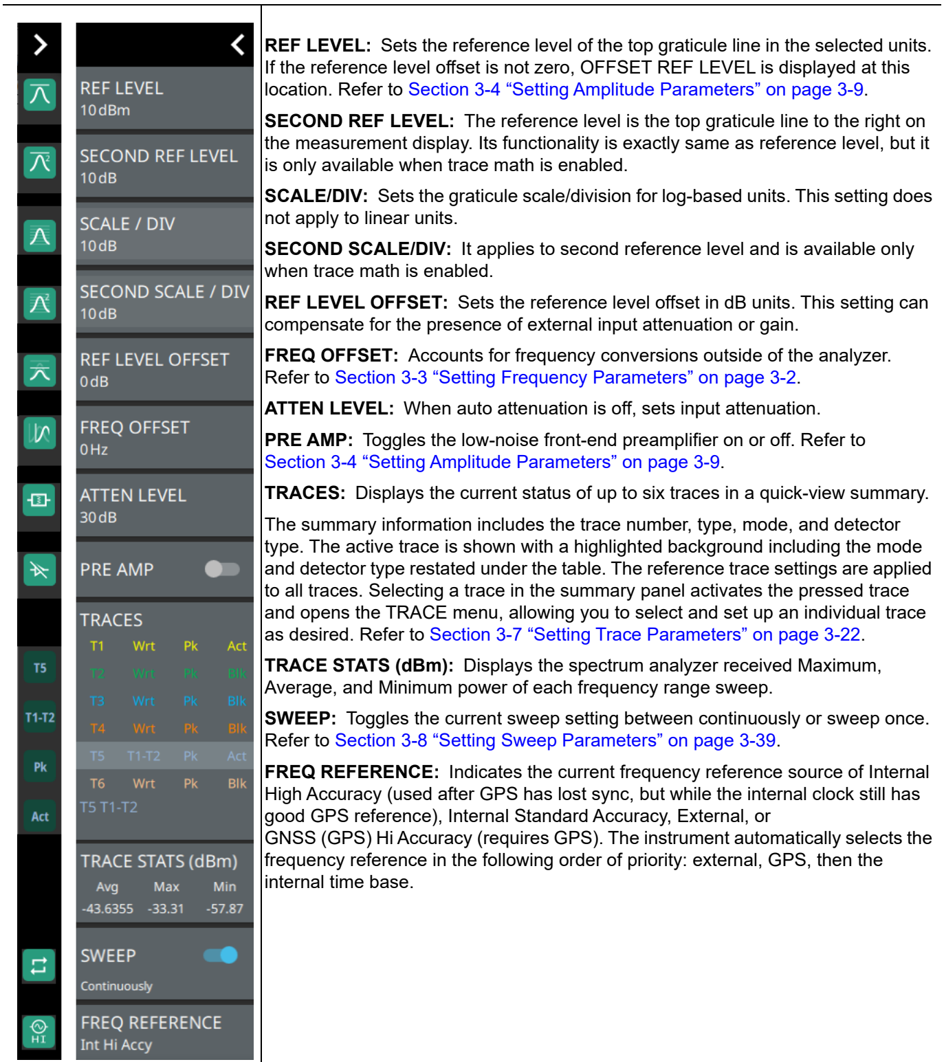
Figure 3-65. Status Panel with Minimized Status Panel Icons (THD)
