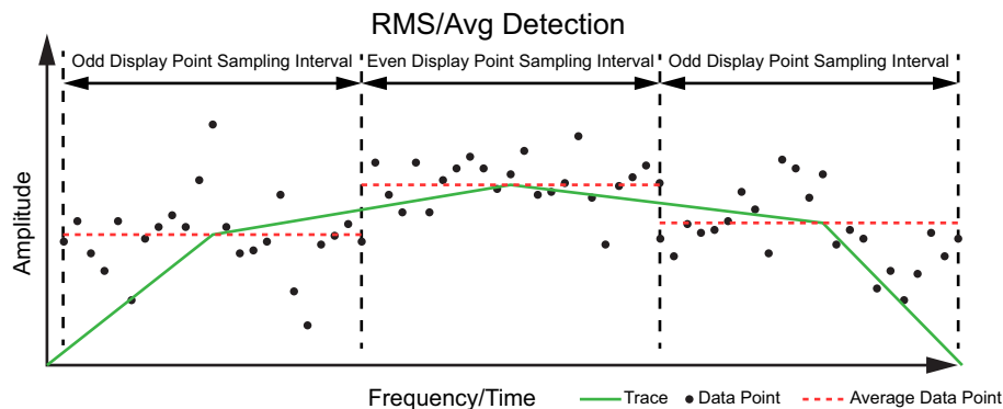
Figure 3-17. RMS/Avg Detector Type
