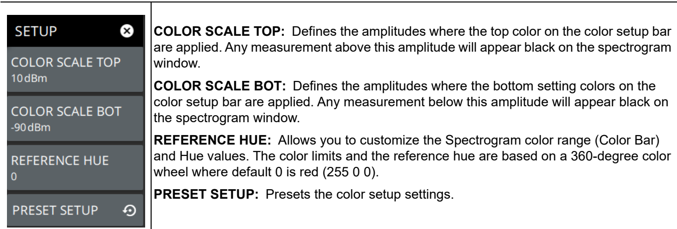
Figure 3-110. SETUP Menu (Spectrogram View)
