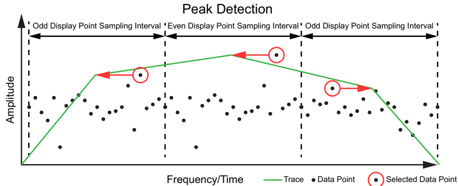
Figure 3-16. Peak Detector Type
