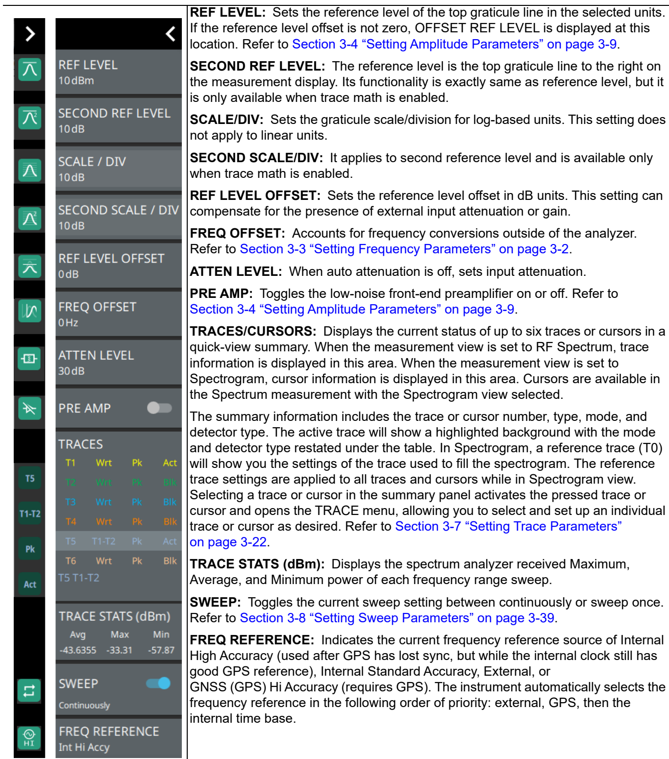
Figure 3-68. Status Panel with Minimized Status Panel Icons (Channel Power)
