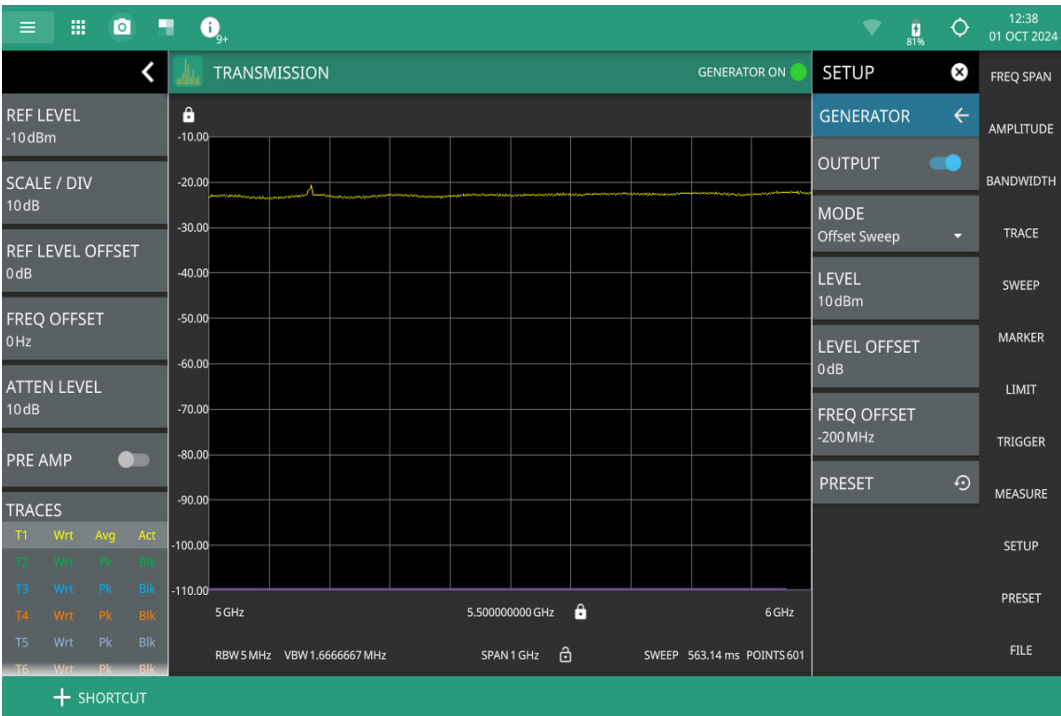
Figure 3-61. Connection of Mixer as DUT - Transmission Measurement
