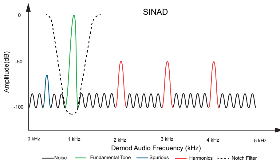
Figure 3-99. SINAD Measurement
