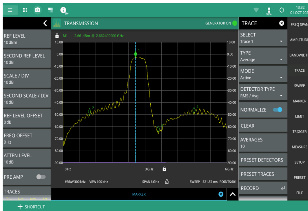
Figure 3-60. Connection of Bandpass Filter as DUT - Transmission Measurement
