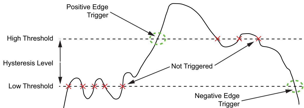
Figure 3-45. Trigger Levels and Hysteresis
