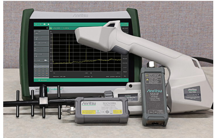
Field Master MS2080A with Power Sensor and Site Master S331P and Handheld InterferenceHunter™ MA2700A
