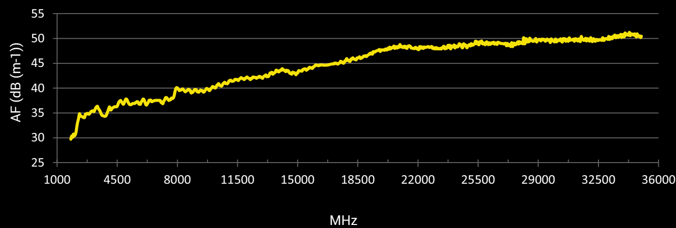
Antenna Factor Diagram HyperLOG® PRO 18350
