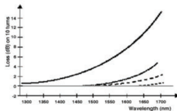
Figure 2-8. Ten wraps on a mandrel produce this type of curve for several types of optical fiber
