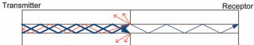
Figure 2-2. A) insertion loss B) optical return loss
