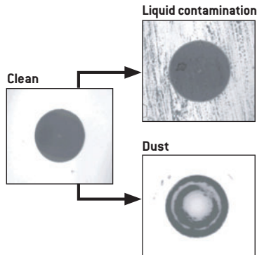
Figure 2-4. Example of soiled connector endfaces
