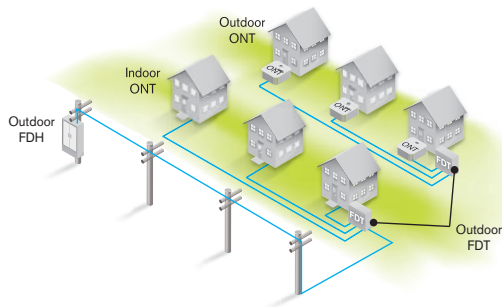
Figure 1-10. Horizontal/garden-style MDU
