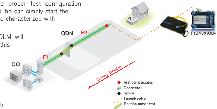
Figure 3-18. iOLM testing
