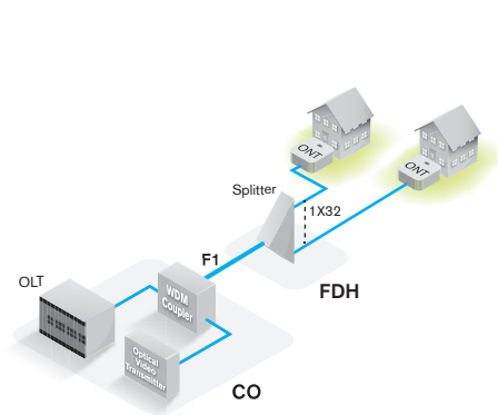
Figure 1-2. Single-stage architecture
