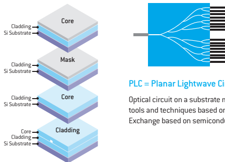
Figure 1-5. Planar waveguide splitter
