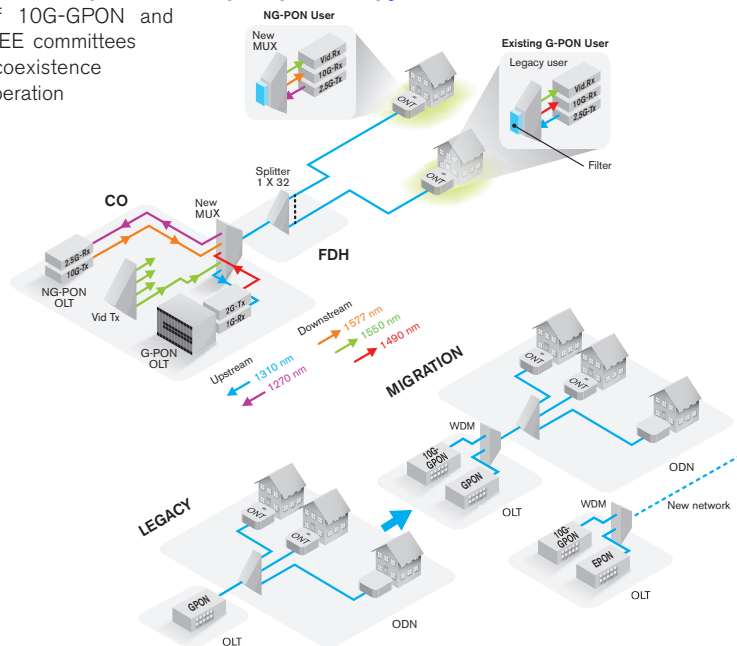
Figure 8-4. Technology coexistence
