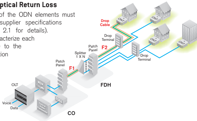
Figure 3-10. Fiber sections in an FTTH ODN
