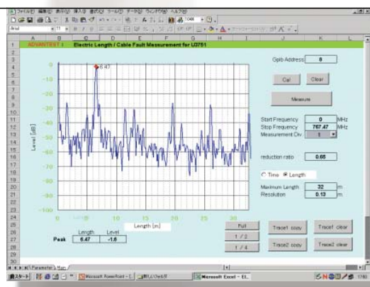
Cable fault point distance measurement
