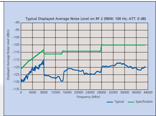
Displayed average noise level (typical)
