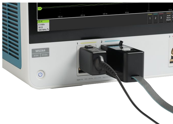
FlexChannel technology enables the ultimate in flexibility. Each input can be configured as a single analog or eight digital channels based on the type of probe you attach.
