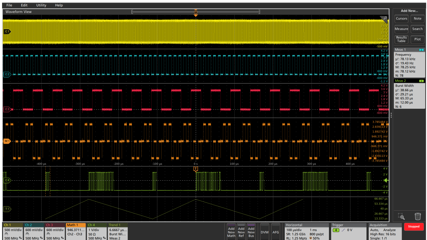
Using measurements to characterize burst width and Frequency.
