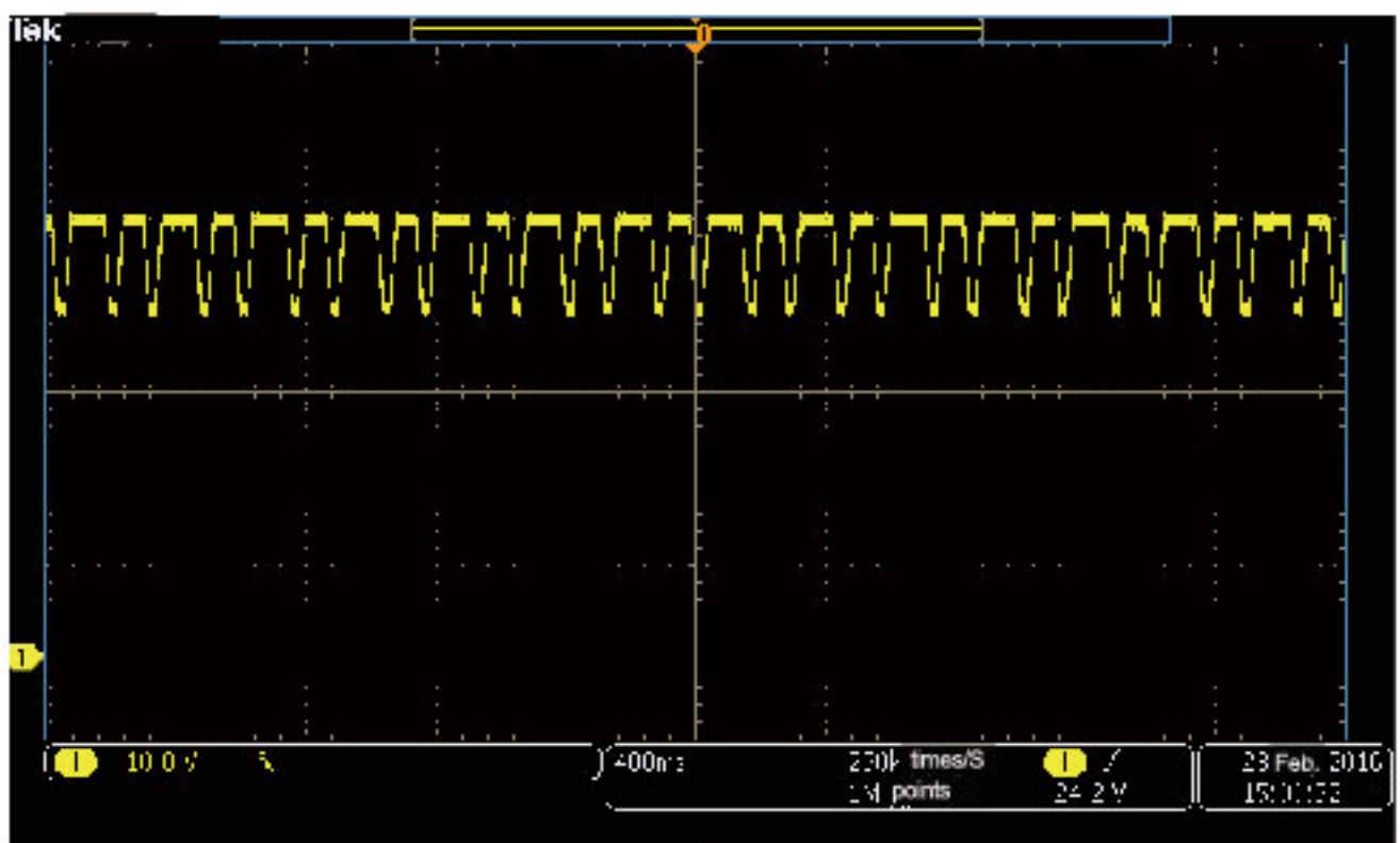
Line Regulation Testing
