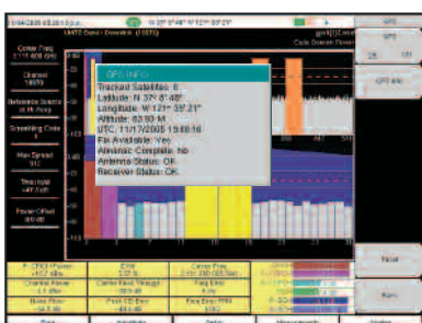
The MT8222A can easily enhance the frequency reference oscillator accuracy to make precise frequency error measurements.
