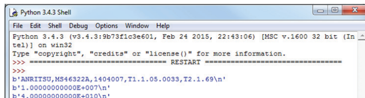
Figure 1-6. Python Script with SCPI Commands for the MS46122A
