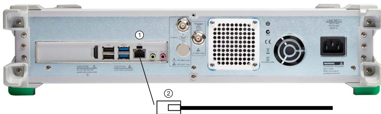
Figure 1-1. Network Connection to MS46322A
