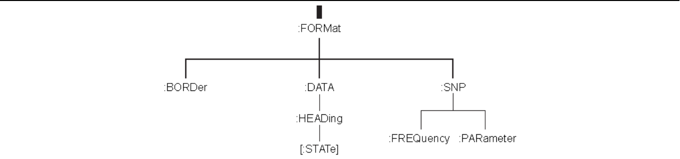
Figure 2-2. SCPI :FORMat Subsystem
