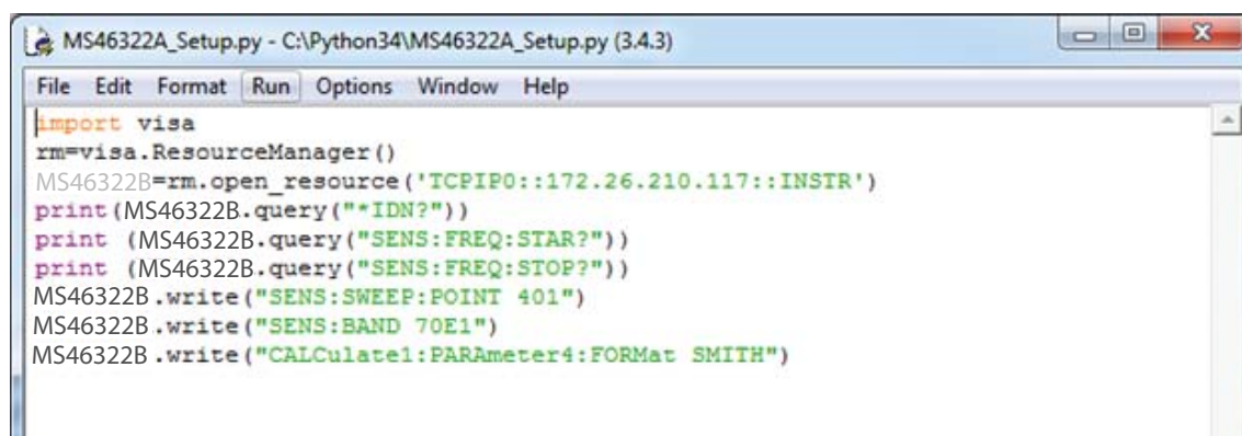
Figure 1-12. Python Script with SCPI Commands
