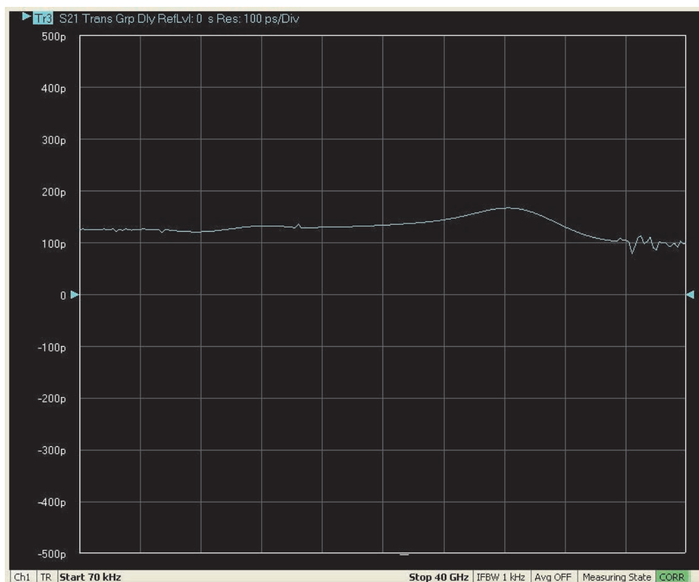
Figure 4-18. Group Delay Trace Graph Example
