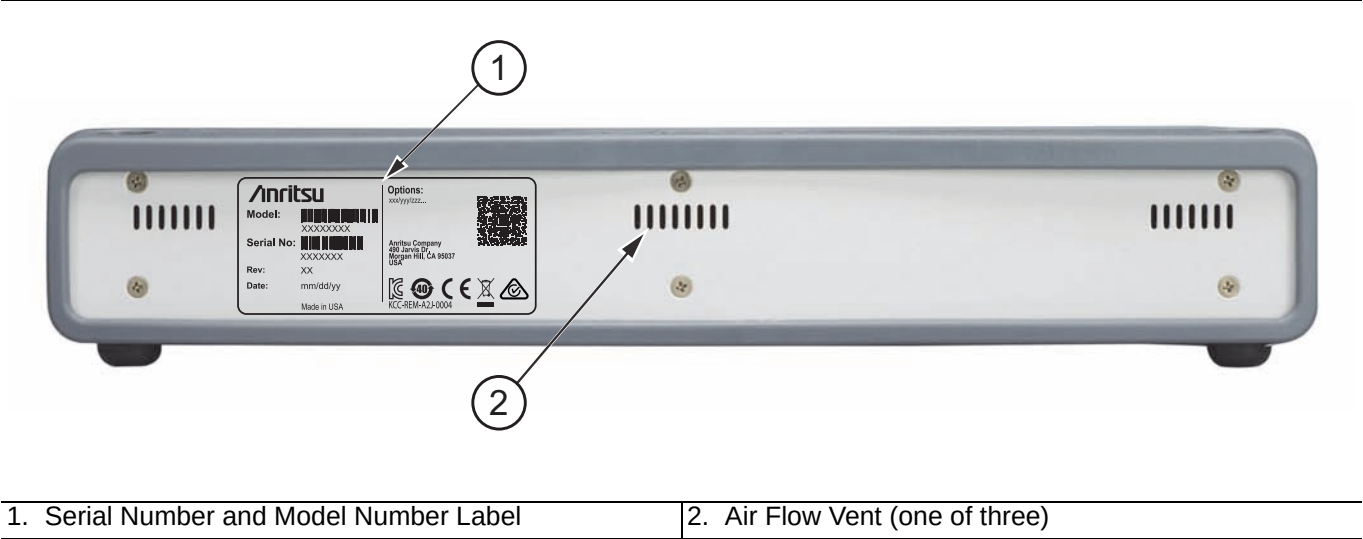
Figure 3-2. MS46122A/B Rear Panel
