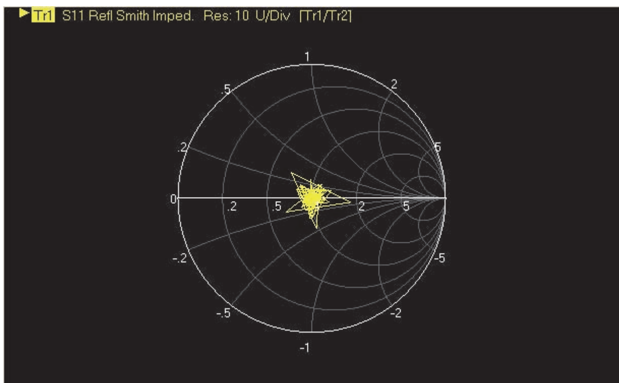
Figure 4-16. Smith Chart with Impedance ( R+jX )
