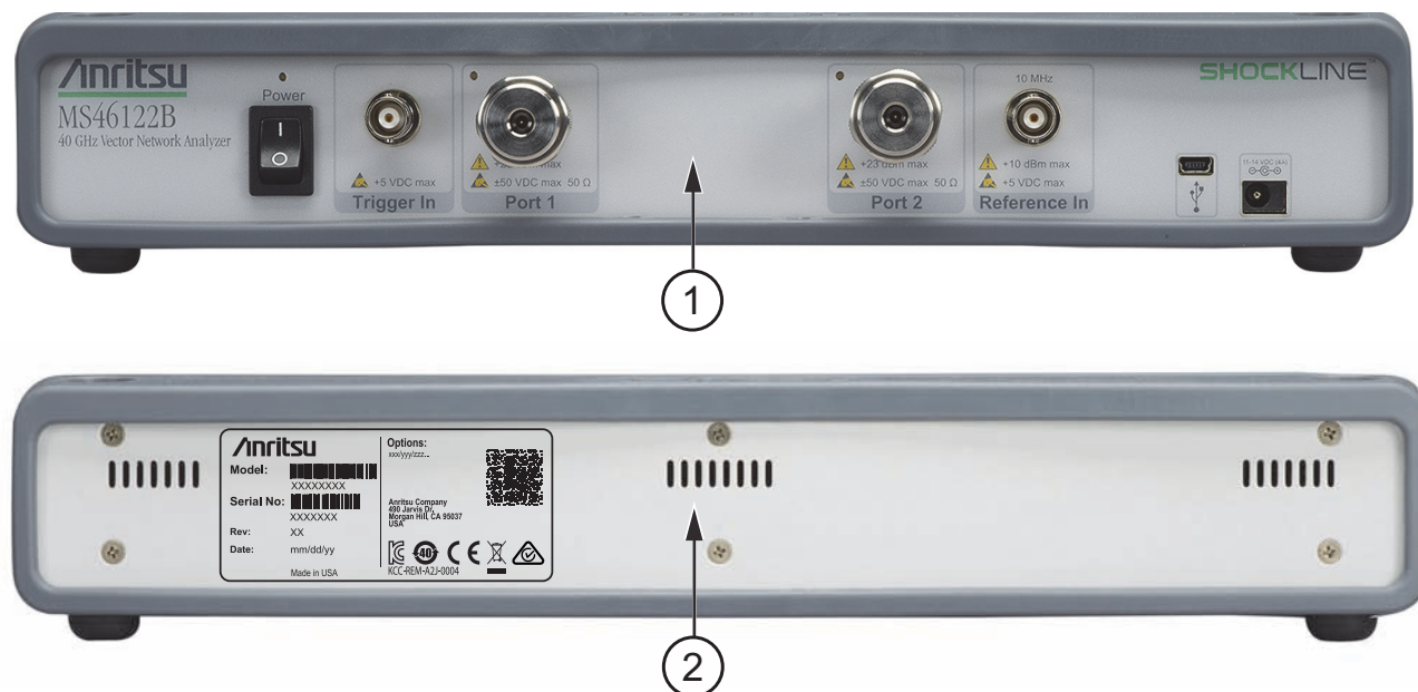
Figure 2-3. MS46122A/B Front Panel and Rear Panel
