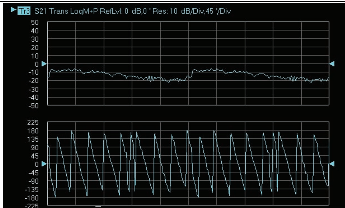
Figure 4-15. Trace Graph - Rectilinear Paired - Trace Log Magnitude and Phase Trace Display
