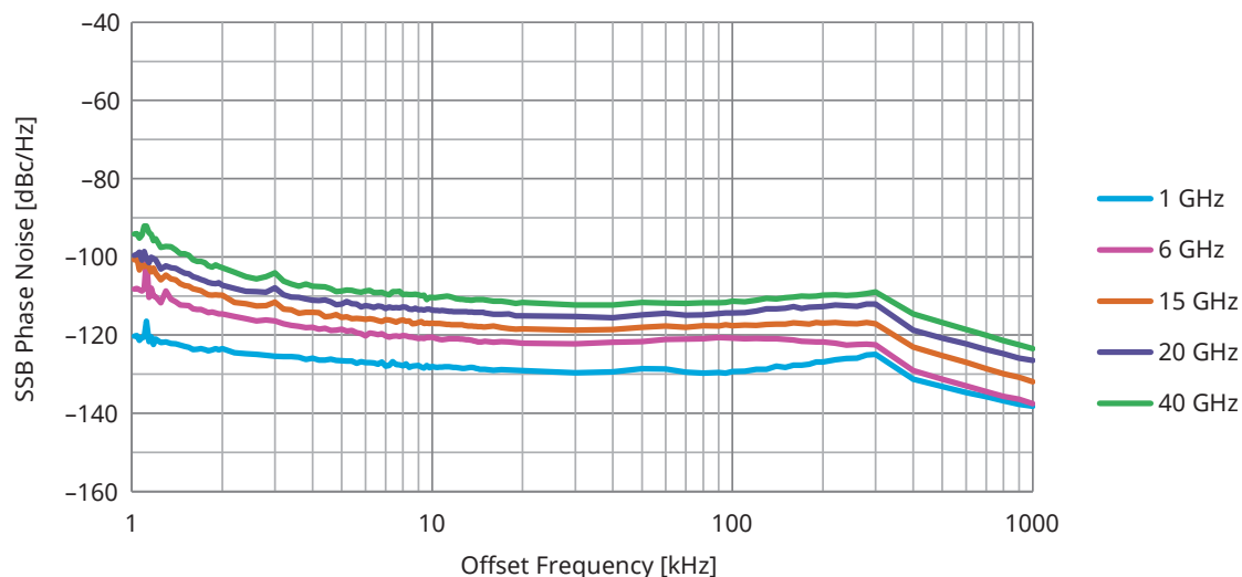
SSB Phase Noise without MS2840A-066 (meas.)
