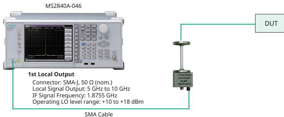
Connection Setup
