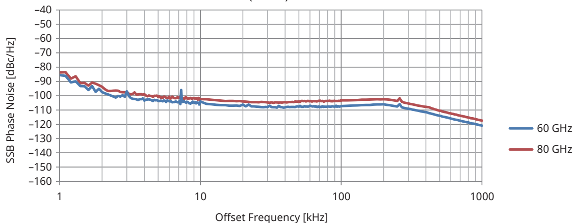
SSB Phase Noise with High Performance Waveguide Mixer (meas.)
