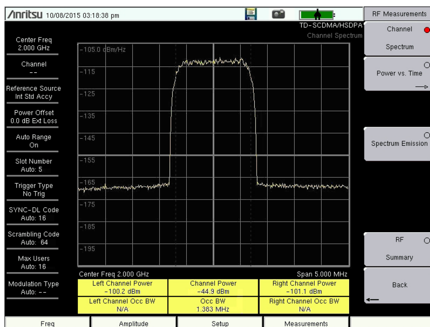
Figure 4-1. TD-SCDMA/HSDPA Channel Spectrum
