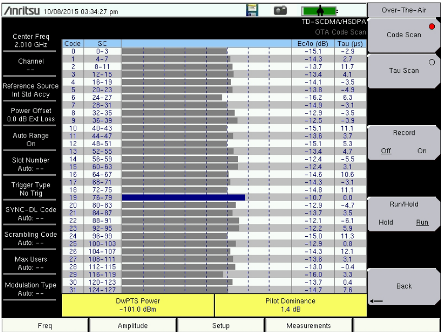
Figure 4-5. TD-SCDMA/HSDPA OTA Code Scan
