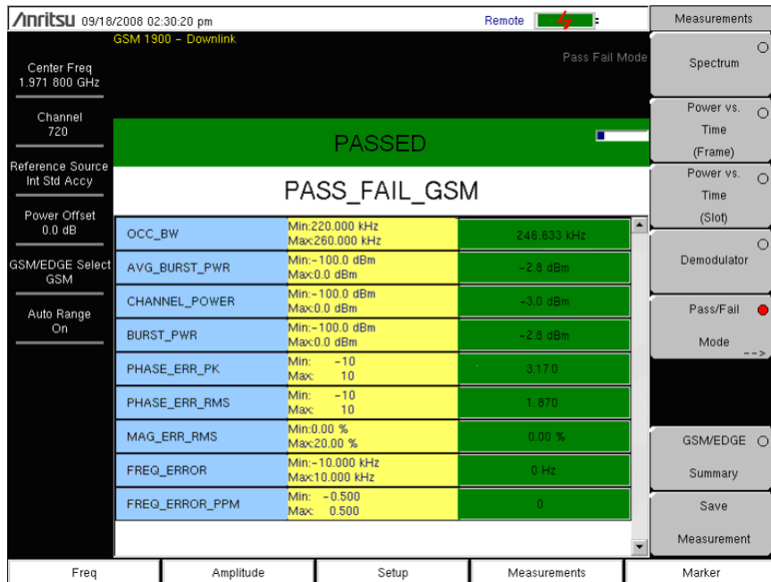
Figure 2-8. Pass/Fail Mode
