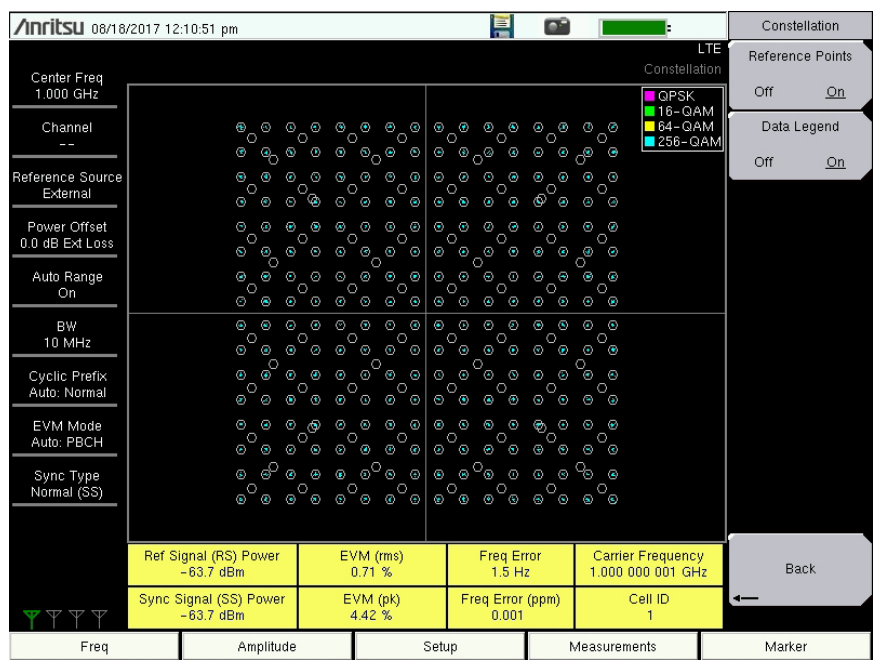
Figure 5-7. Constellation Measurement View
