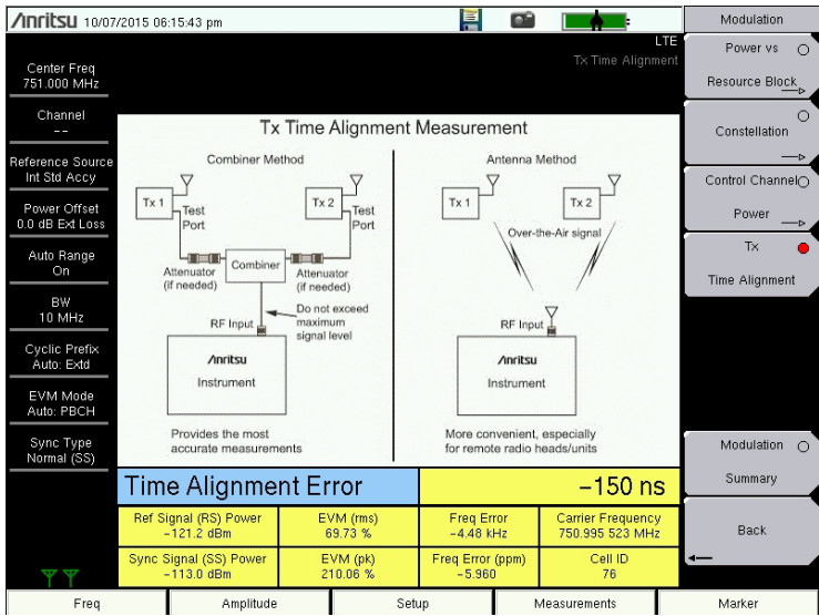
Figure 5-10. Tx Time Alignment
