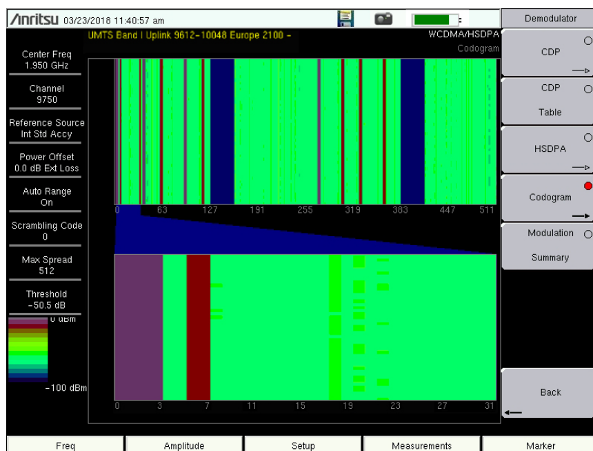
Figure 3-10. Codogram Measurement
