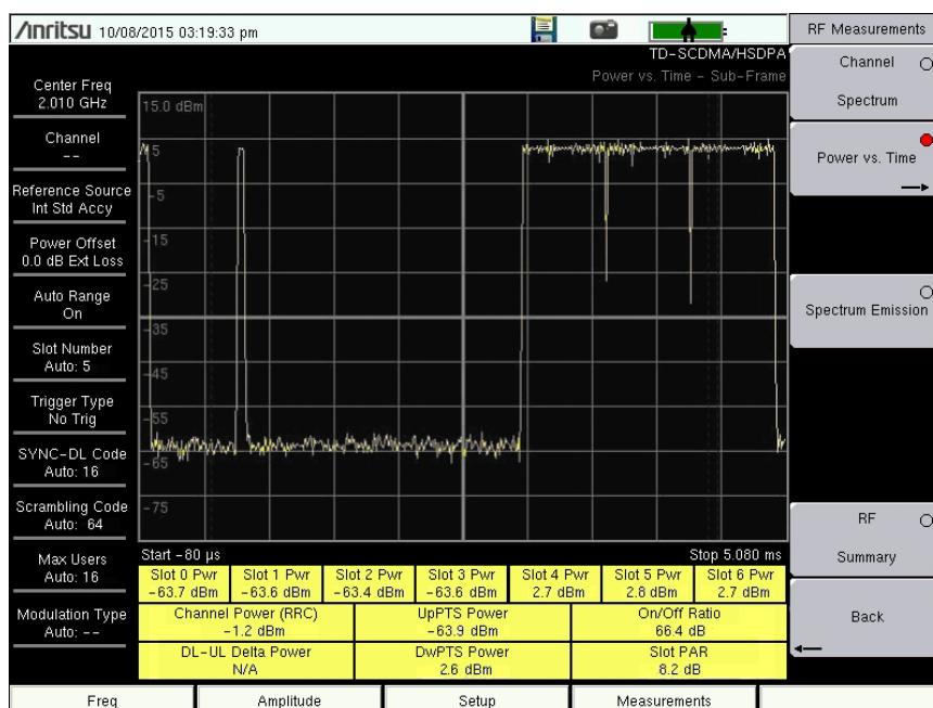
Figure 4-2. TD-SCDMA/HSDPA Power vs. Time: Sub-Frame Measurement
