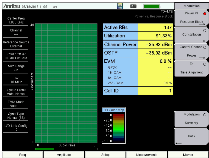
Figure 6-7. Power vs Resource Block Measurement View
