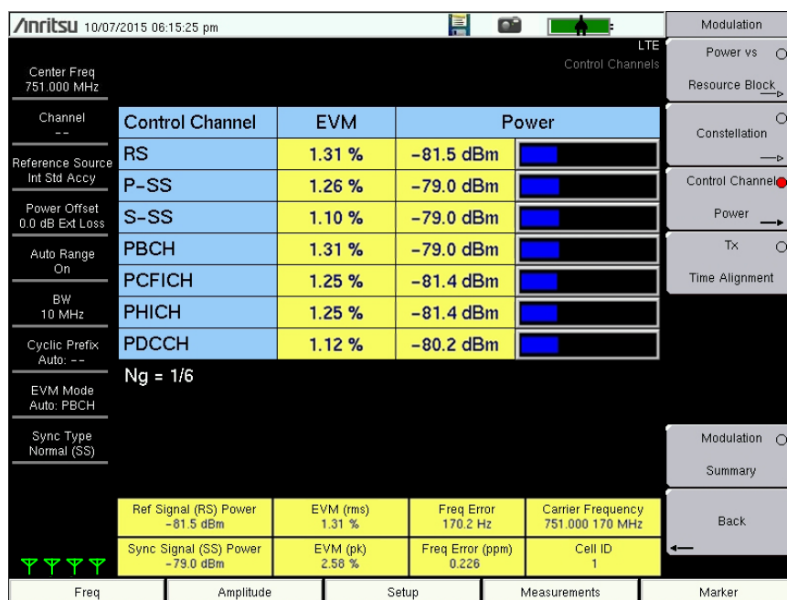
Figure 5-8. Control Channel Power
