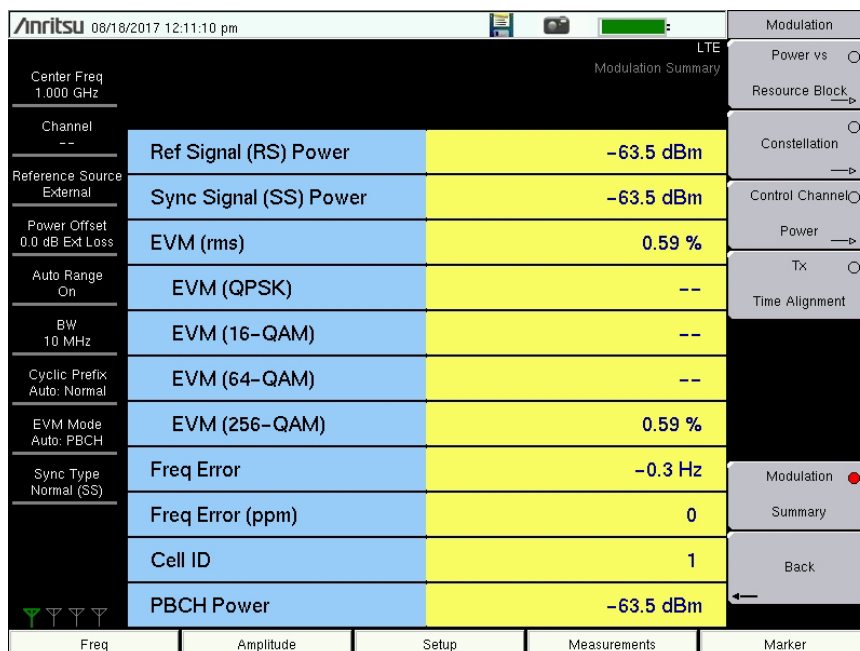
Figure 5-11. Modulation Summary
