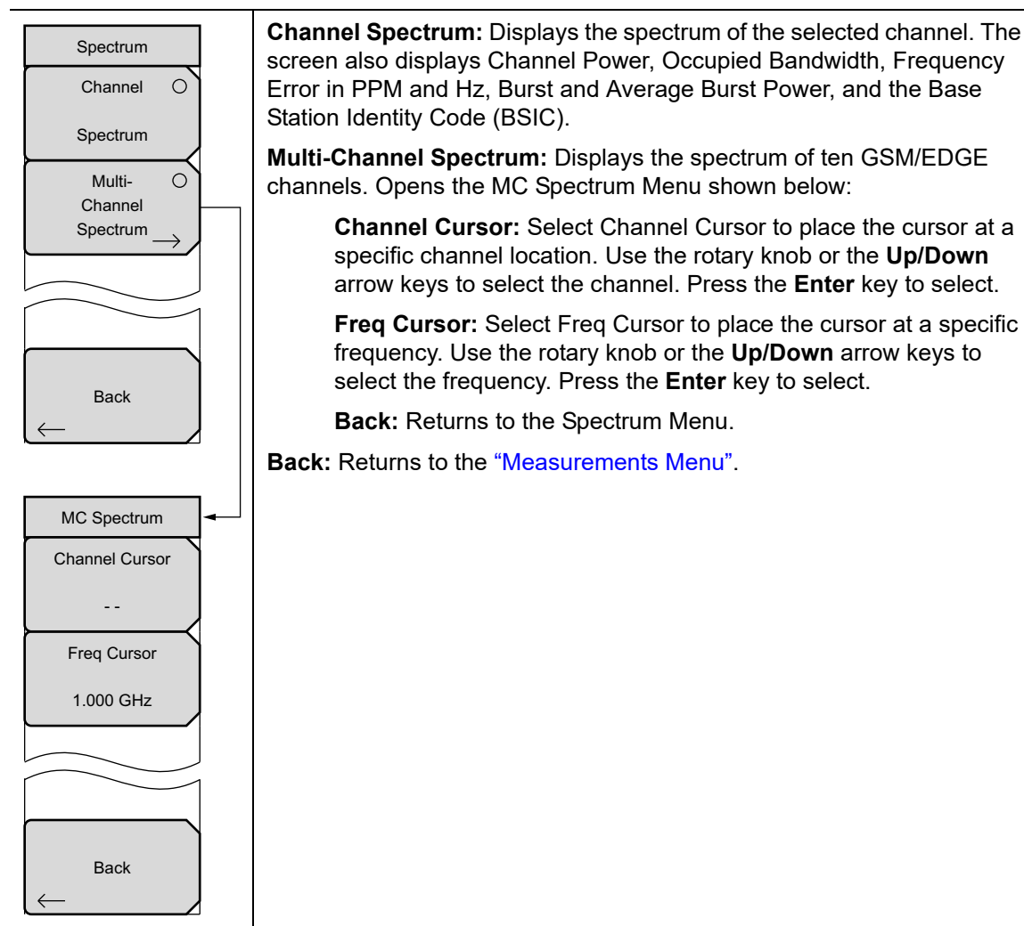
Figure 2-14. Spectrum Menu
