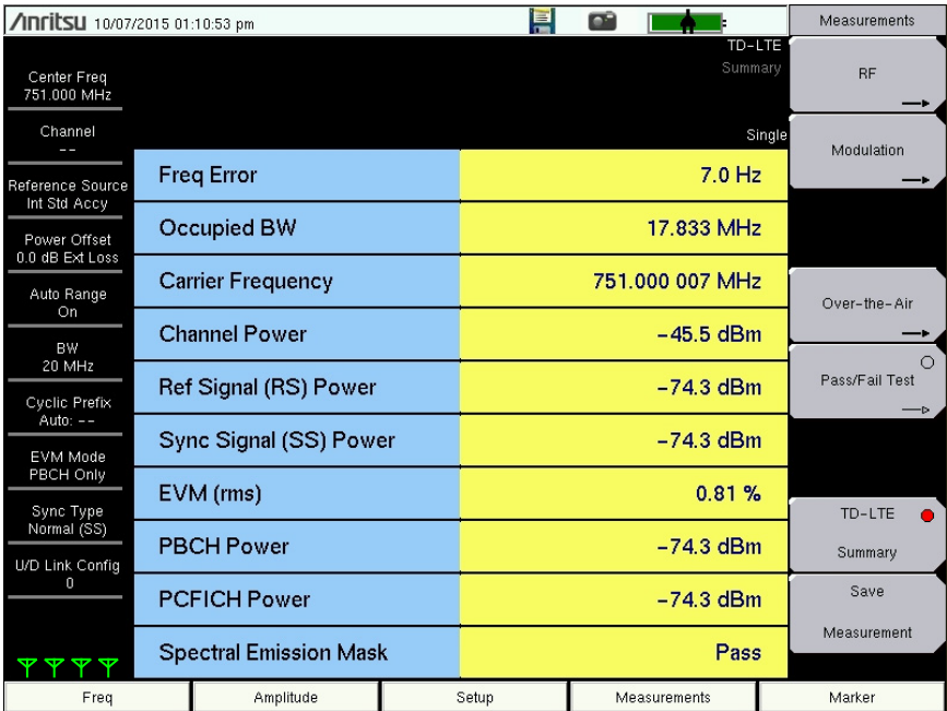
Figure 6-17. TD-LTE Summary
