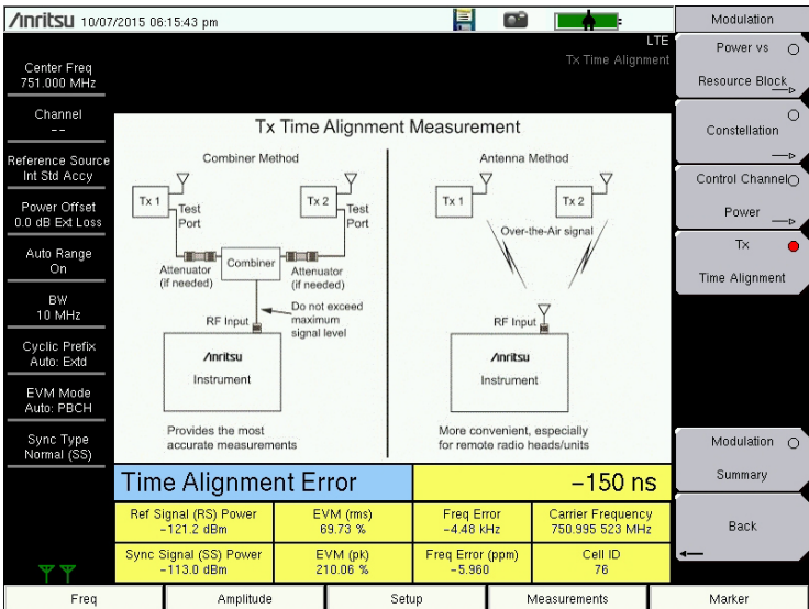
Figure 6-11. Tx Time Alignment
