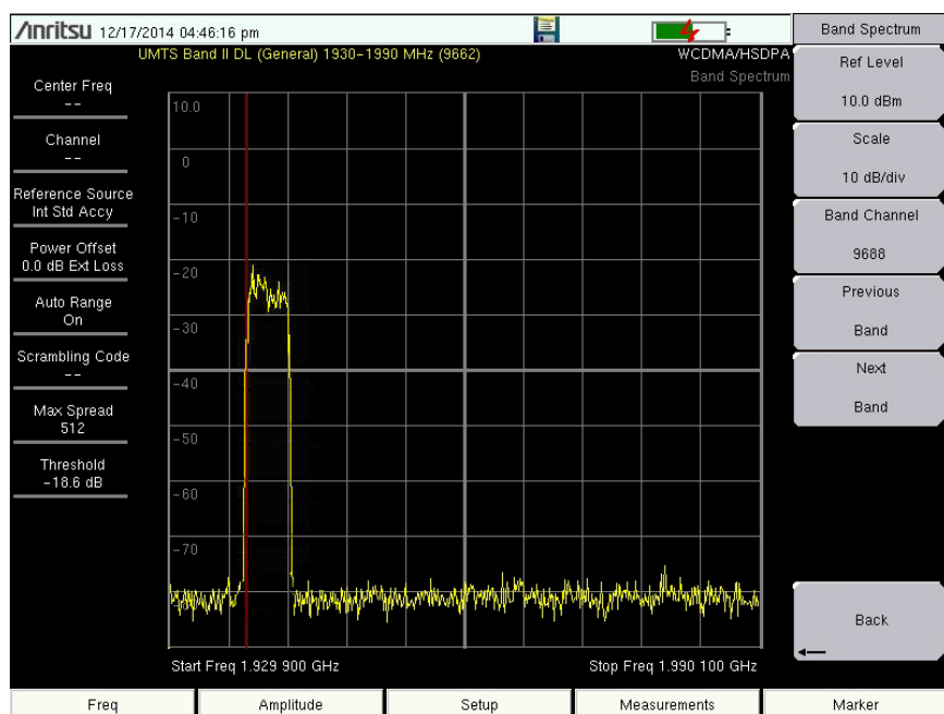
Figure 3-1. Band Spectrum
