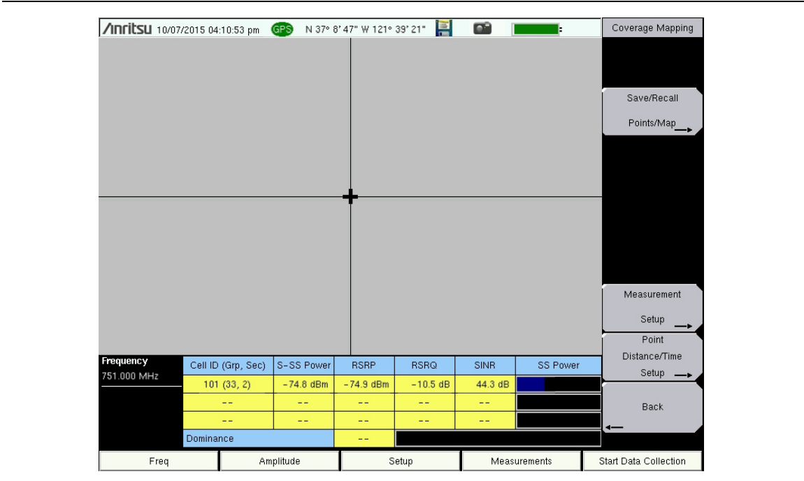
Figure 7-3. LTE Coverage Mapping with the Default Grid
