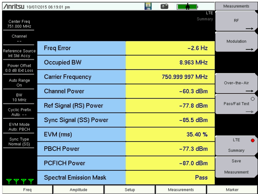
Figure 5-16. LTE Summary
