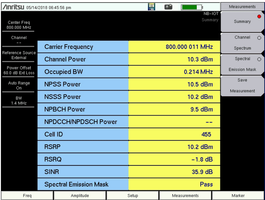
Figure 8-1. NB-IoT Summary
