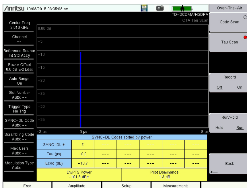
Figure 4-6. TD-SCDMA/HSDPA OTA Tau Scan
