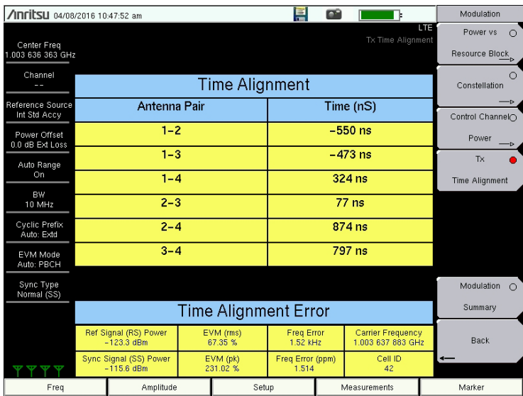
Figure 5-9. Tx Time Alignment (4x4 MIMO Configuration)
