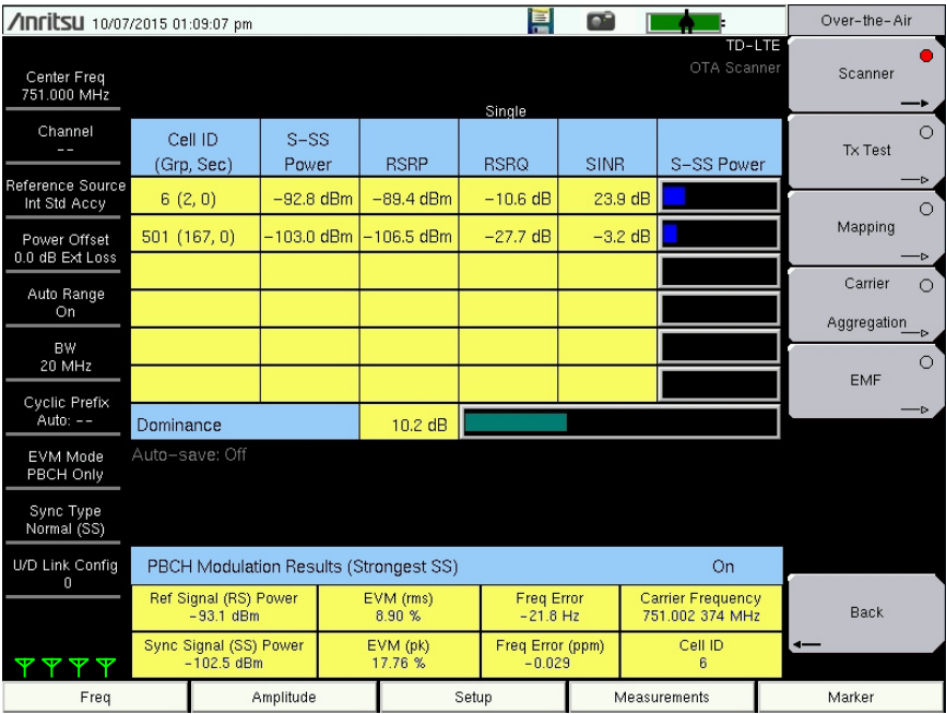
Figure 6-13. Over-the-Air Measurements
