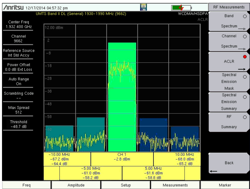
Figure 3-3. ACLR Measurement
