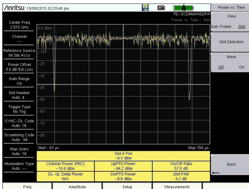
Figure 4-3. TD-SCDMA/HSDPA Power vs. Time: Slot Measurement
