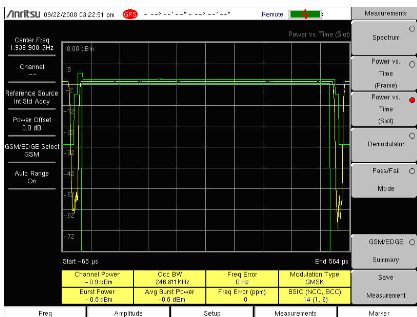
To display Power versus Time (Slot) press the Power versus Time (Slot) submenu key to activate the Power versus Time (Slot) measurement ( Figure 2-4 ). The mask is according to the 3GPP TS 05.05 specification. The first slot information is displayed.
