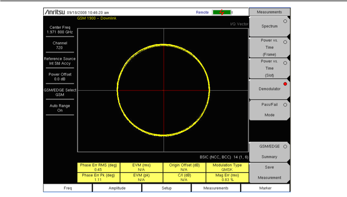
Figure 2-5. GSM Demodulator Measurement
