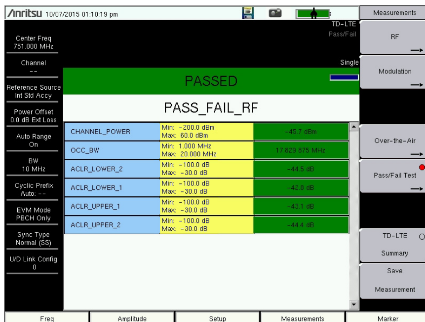
Figure 6-16. Past/Fail Test
