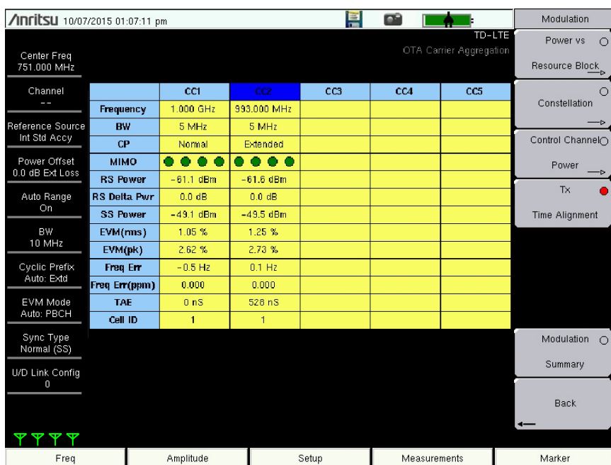
Figure 6-15. Over-the-Air Carrier Aggregation Measurement
