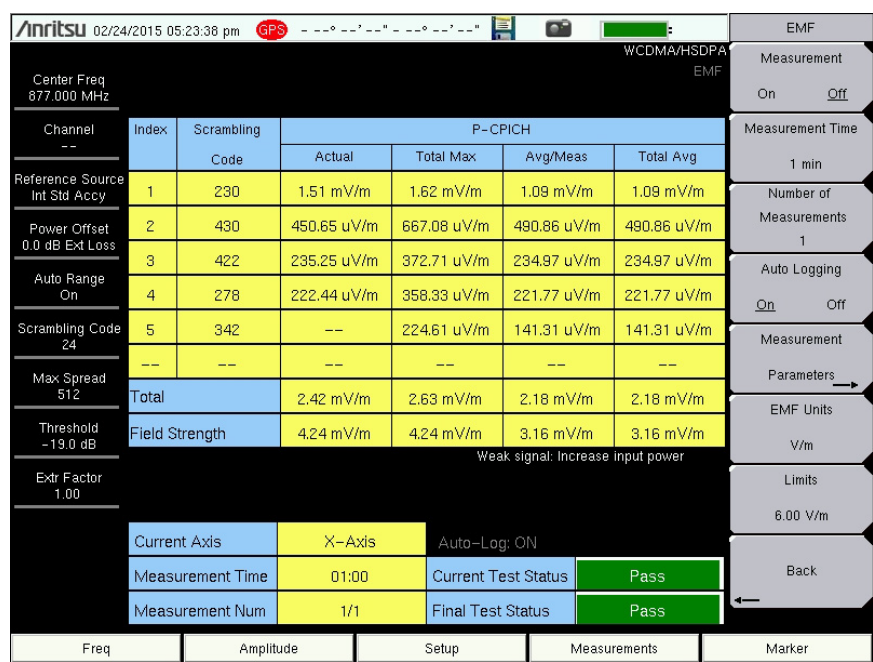
Figure 9-13. W-CDMA EMF Measurement Results
