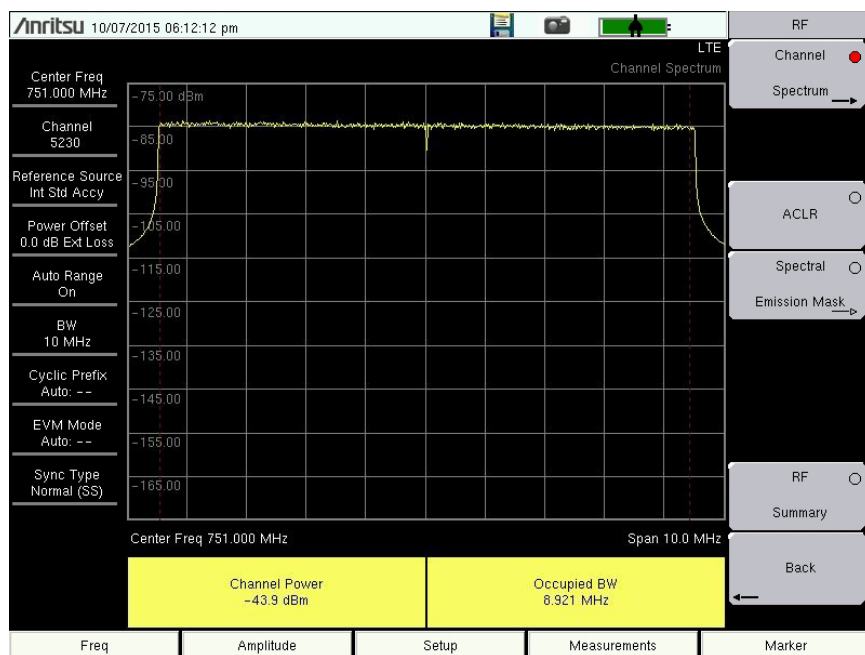
Figure 5-2. Channel Spectrum
