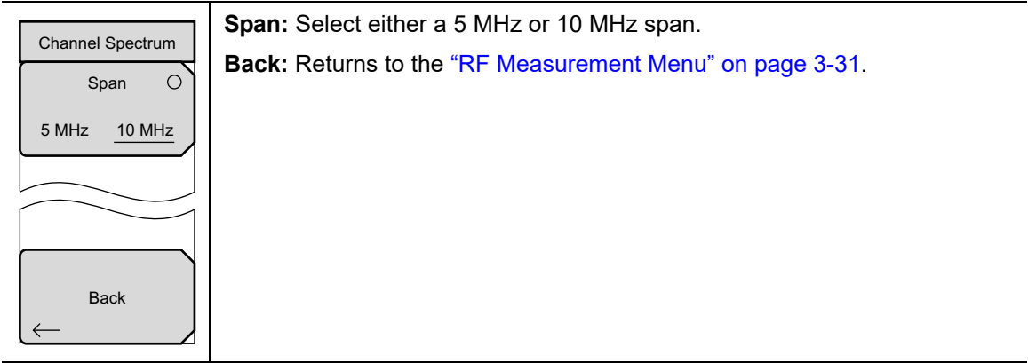
Figure 3-23. W-CDMA/HSDPA Channel Spectrum Menu
