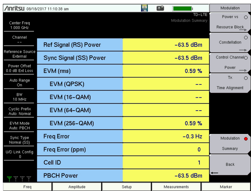
Figure 6-12. Modulation Summary
