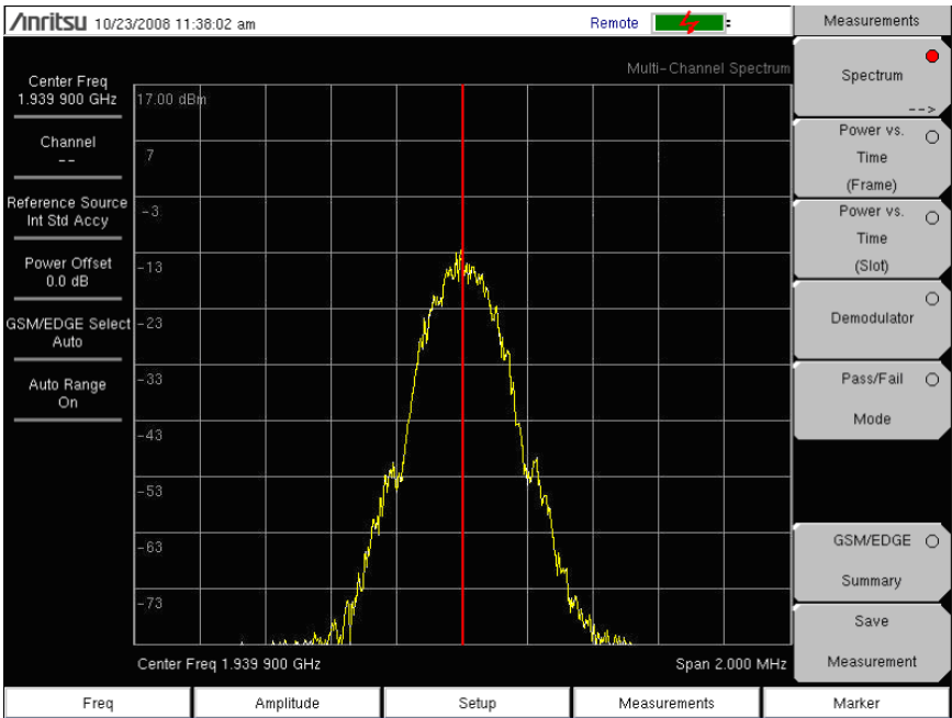
Figure 2-2. GSM Multi-Channel Measurement
