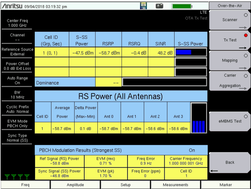
Figure 5-13. Over-the-Air Tx Test Measurement
