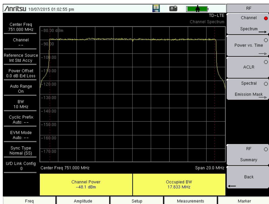
Figure 6-2. Channel Spectrum
