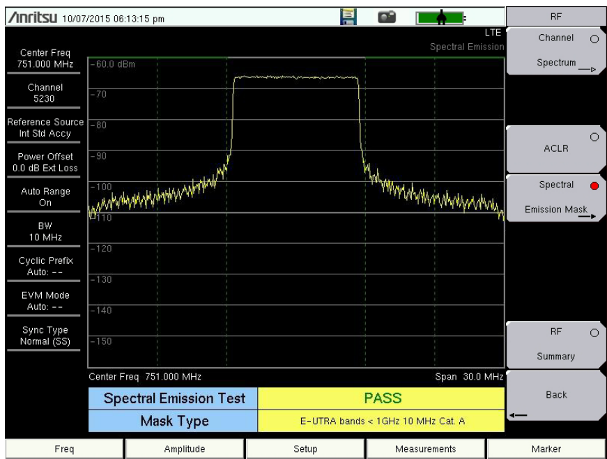
Figure 5-4. Spectral Emission Mask
