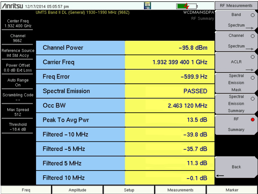
Figure 3-7. RF Summary
