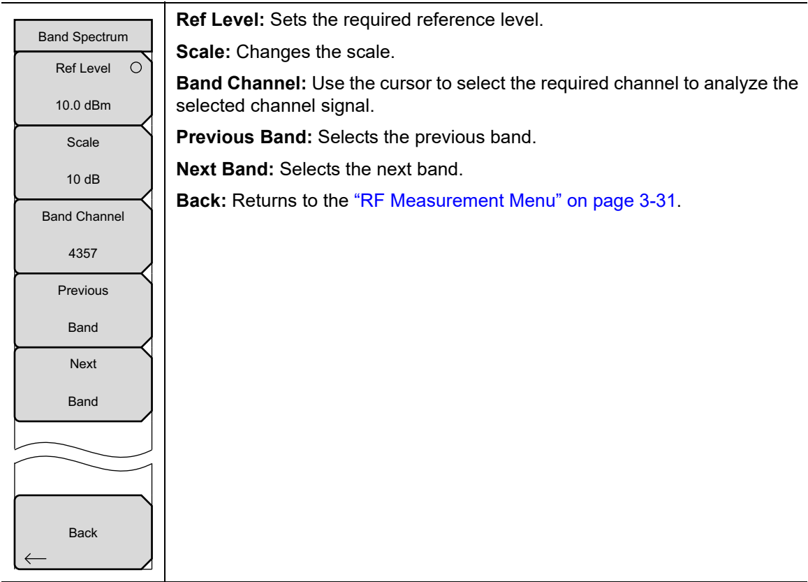
Figure 3-22. W-CDMA/HSDPA Band Spectrum Menu
