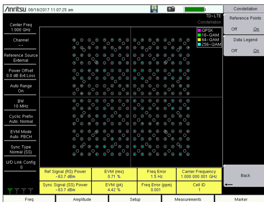
Figure 6-8. Constellation Measurement View
