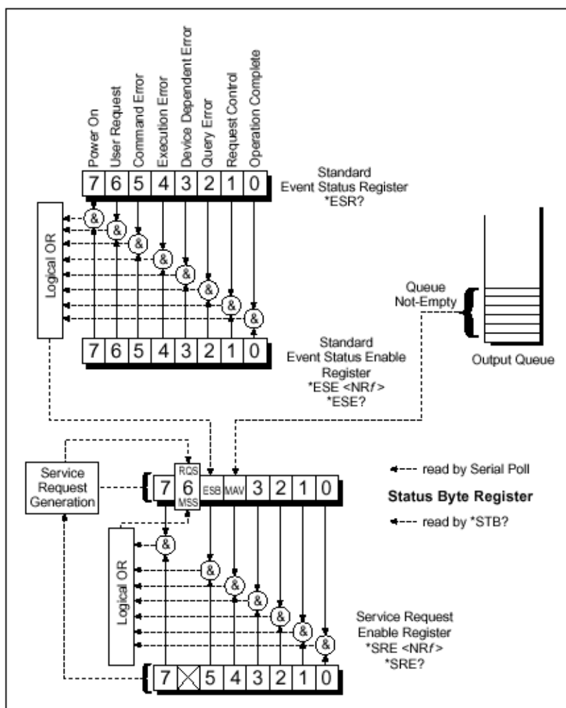
Figure 2-3. Status Byte Register
