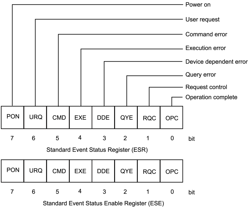
Figure 2-2. Standard Event Status Enable Register
