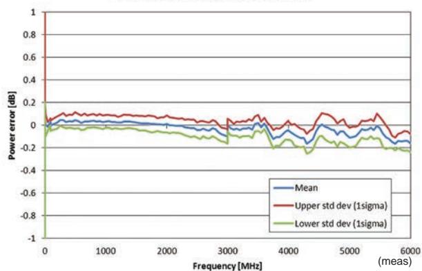
Frequency Characteristic
