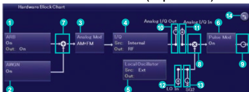
Hardware Block Chart (Explanation)
