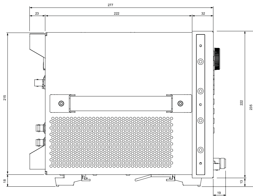
Figure 12. Dimensions (side view, in millimeters)
