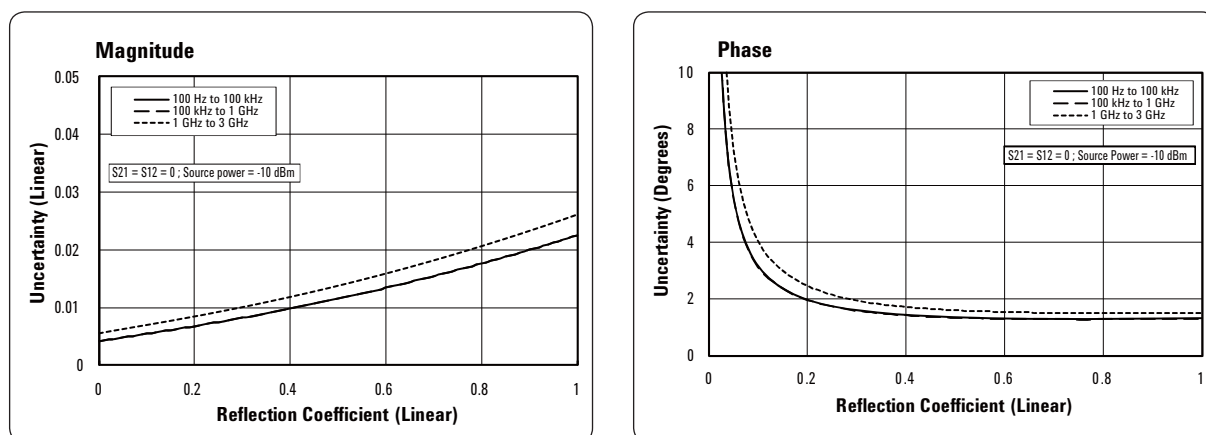
Figure 2. Reflection uncertainty (specification)
