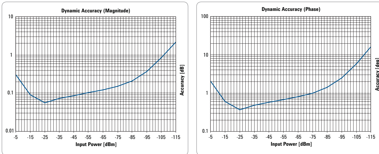
Figure 9. Dynamic Accuracy
