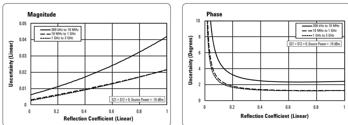
Figure 6. Reflection uncertainty (specification)
