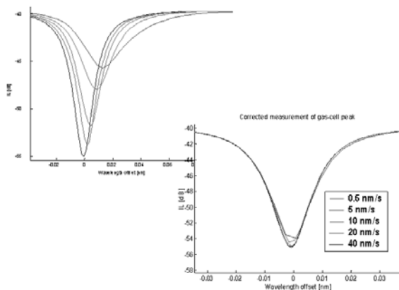
Correction algorithm for spectrum characterization
