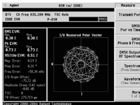
E4440 PSA screen image showing an EDGE constellation diagram generated by the E4438C ESG.
