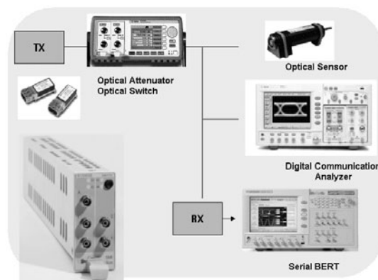
Solution for system integration using optical switch
