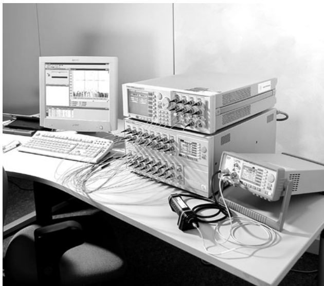
40ch spectrum analysis synchronizing tunable laser source and power meter
