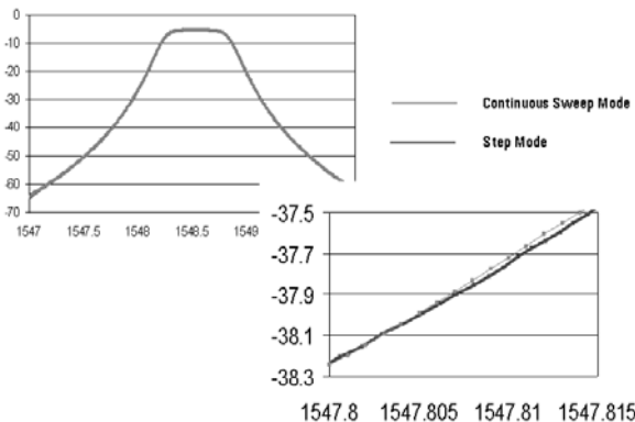
No compromise on sweep speed
