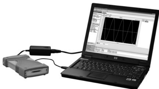
The U2300A data acquisition device setup in standalone operation.
