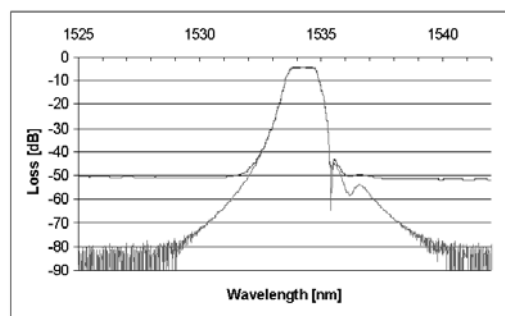
Agilent's spectrum analysis solution compared with conventional solution
