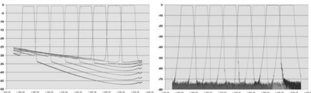
Low SSE and high power measurement result
