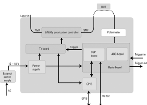
N7788A PMD / PDL component analyzer setup
