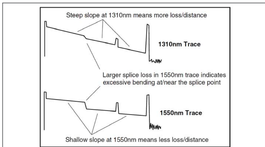
Figure 10 - Wavelength Differences
