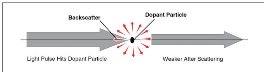
Figure 2 - Rayleigh Scattering
