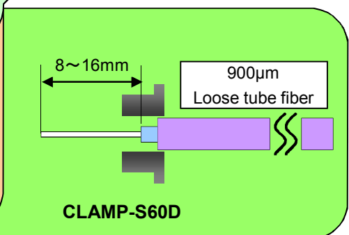
Setting onto splicer
