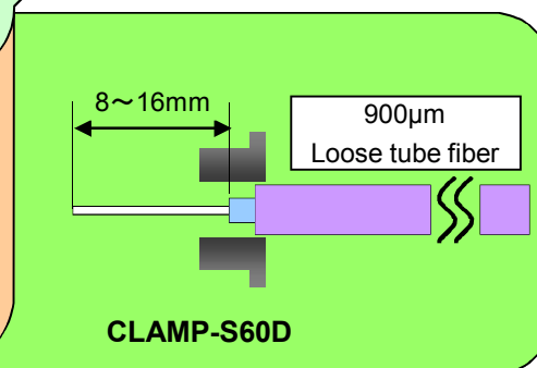
Setting onto splicer
