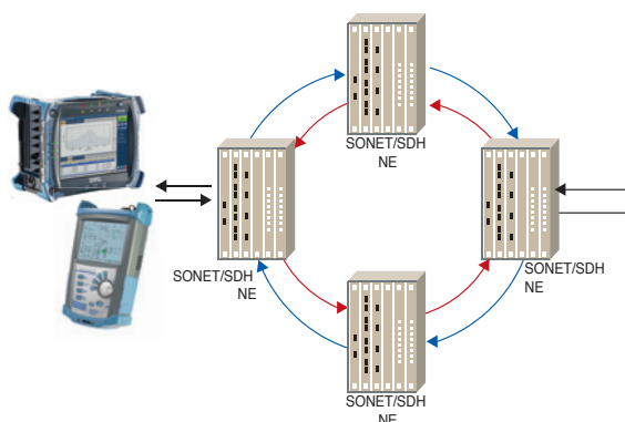
Housed in the FTB-500 or FTB-200 platform, the FTB-8115 module enables field circuit turn-up and troubleshooting.
