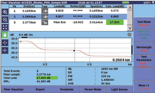
PON Measurement Analysis Screen
