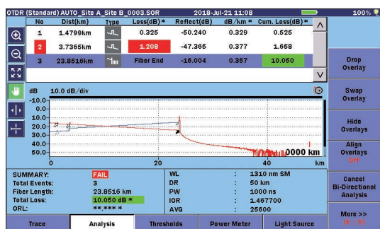
Bi-directional Analysis Screen
