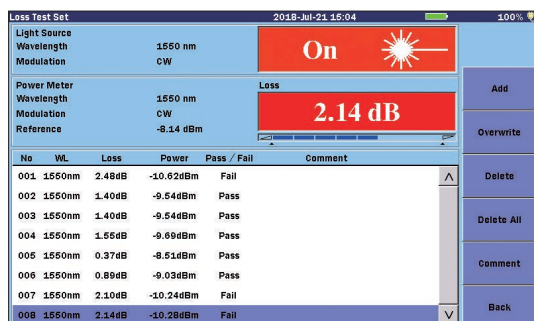
Logged Optical Power and Loss Output Screen
