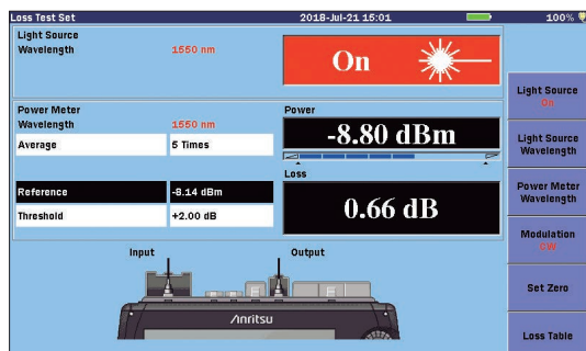
Optical Loss Measurement
