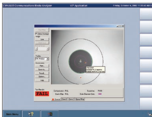
Video Inspection Probe displays and captures fiber end face
