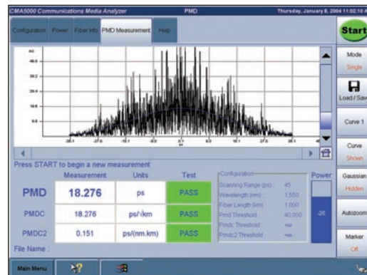
Determine if your fiber link meets PMD requirements
