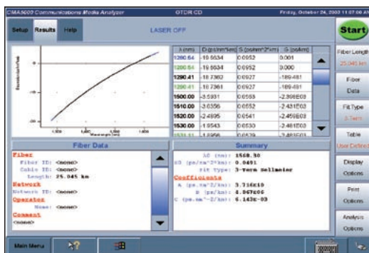
Highly Accurate CD Measurement Using FOTP-168 Method
