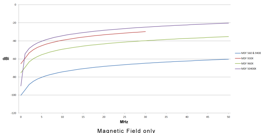
Antenna Gain
